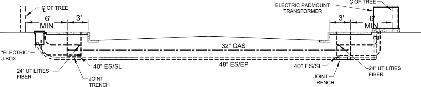
TRENCH PROFILE & STREET CROSSING VIEW (50' R.O.W. AND 6' SIDEWALKS)
