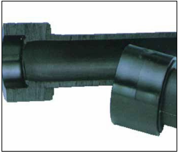
Excessive Stab Depth Caused by Failure to Use a Cold Ring
