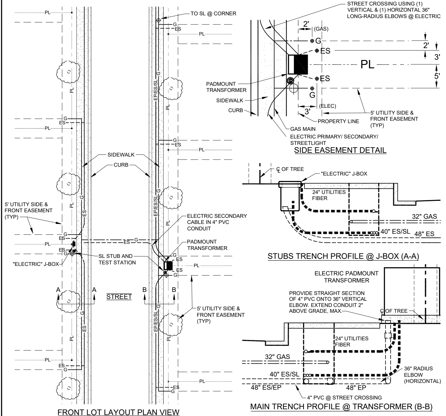
FRONT LOT LAYOUT PLAN VIEW
